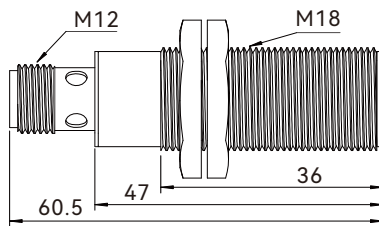
CSB18 series J45
