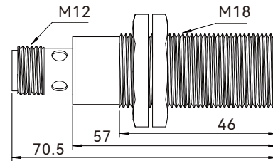
CSB18 series J55
